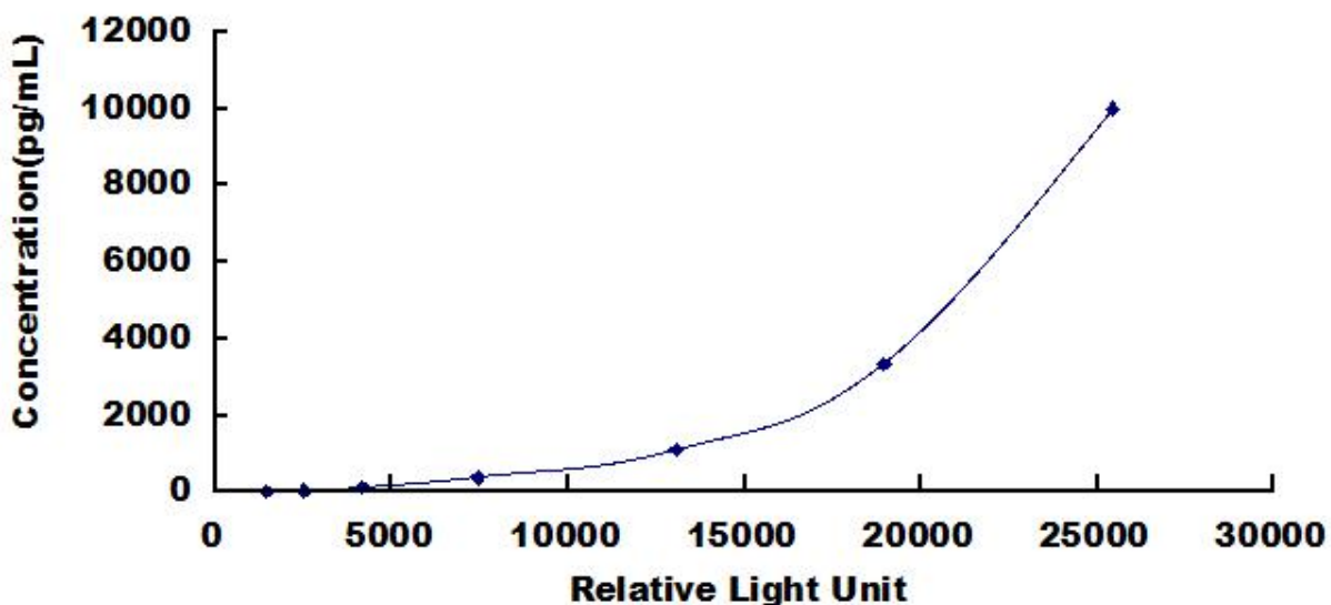
Typical Standard Curve for H4 CLIA.
