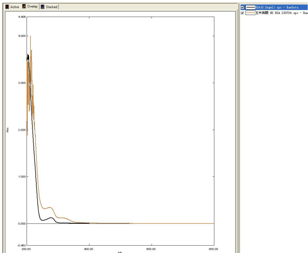
Figure 1. UV-spectrum
