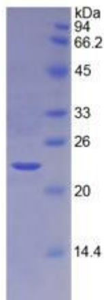
Figure 2. SDS-PAGE
