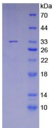
Figure 2. SDS-PAGE
