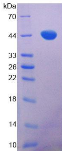
Figure 2. SDS-PAGE
