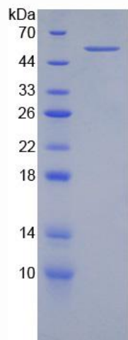
Figure 2. SDS-PAGE
