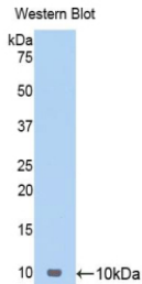
Figure. Western Blot; Sample: Recombinant TARC, Human.
