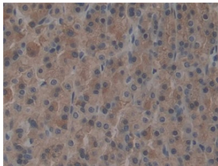
DAB staining on IHC-P; Samples: Rat Stomach Tissue; Primary Ab: 10µg/ml Rabbit Anti-Rat TBX21 Antibody Second Ab: 2µg/mL HRP-Linked Caprine Anti-Rabbit IgG Polyclonal Antibody (Catalog: SAA544Rb19)
