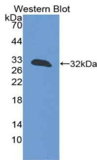
Figure. Western Blot; Sample: Recombinant TBX21, Rat.
