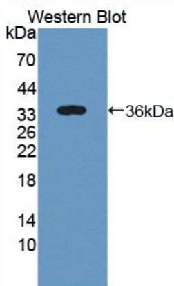
Used in Western Blot, Sample: Recombinant ST2, Human
