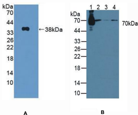
Figure 1. Western Blot
