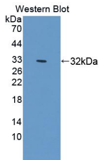
Figure. Western Blot; Sample: Recombinant SIRPa, Mouse.
