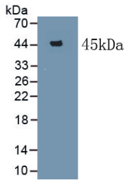
Figure. Western Blot; Sample: Recombinant SAA, Bovine.
