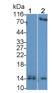
Western Blot; Sample: Lane1: Bovine Liver lysate; Lane2: Human Saliva Primary Ab: 1µg/ml Rabbit Anti-Bovine SAA Antibody Second Ab: 0.2µg/mL HRP-Linked Caprine Anti-Rabbit IgG Polyclonal Antibody (Catalog: SAA544Rb19)
