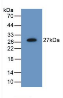
Figure. Western Blot; Sample: Recombinant MB21D1, Mouse.
