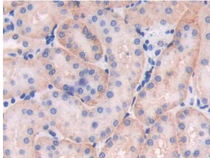
DAB staining on IHC-P; Samples: Mouse Kidney Tissue; Primary Ab: 10µg/ml Rabbit Anti-Mouse MB21D1 Antibody Second Ab: 2µg/mL HRP-Linked Caprine Anti-Rabbit IgG Polyclonal Antibody (Catalog: SAA544Rb19)
