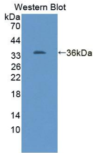
Figure. Western Blot; Sample: Recombinant Kim1, Rat.
