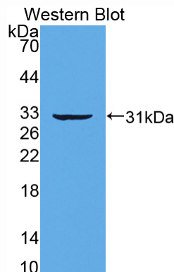
Used in Western Blot, Sample: Recombinant IRF5, Mouse
