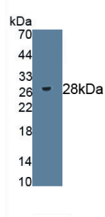
Figure. Western Blot; Sample: Recombinant HSPG2, Mouse.
