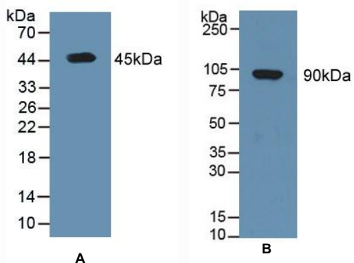
Figure 1. Western Blot
