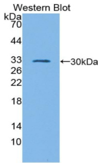
Figure. Western Blot; Sample: Recombinant GATA1, Mouse.
