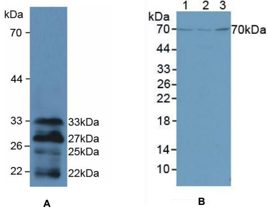
Figure 1. Western Blot
