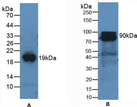
Figure 1. Western Blot
