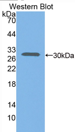
Used in Western Blot, Sample: Recombinant CXCL16, Mouse
