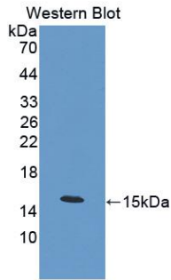
Figure. Western Blot; Sample: Recombinant Calcitonin, Mouse.
