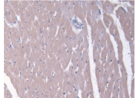
DAB staining on IHC-P; Samples: Rat Heart Tissue; Primary Ab: 20µg/ml Rabbit Anti-Rat ABCC6 Antibody Second Ab: 2µg/mL HRP-Linked Caprine Anti-Rabbit IgG Polyclonal Antibody (Catalog: SAA544Rb19)
