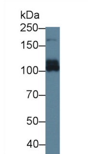
Western Blot; Sample: Rat Liver lysate; Primary Ab: 1µg/ml Rabbit Anti-Rat ABCC6 Antibody Second Ab: 0.2µg/mL HRP-Linked Caprine Anti-Rabbit IgG Polyclonal Antibody (Catalog: SAA544Rb19)
