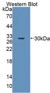
Figure. Western Blot; Sample: Recombinant ABCC6, Rat.
