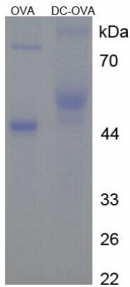
Figure 1. SDS-PAGE
