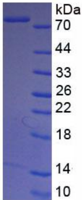
Figure 1. SDS-PAGE
