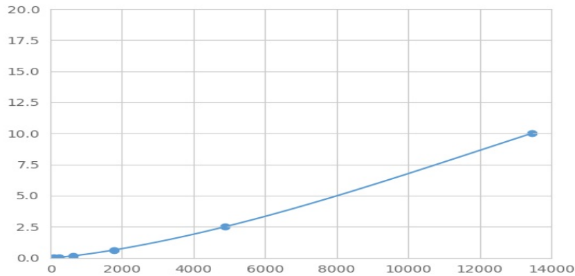
Typical Standard Curve for TLR10 Magnetic Luminex Assay.
