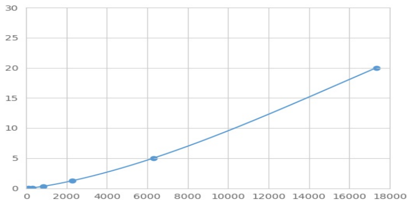
Typical Standard Curve for TIRAP Magnetic Luminex Assay.
