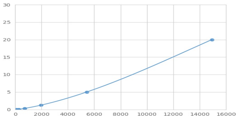
Typical Standard Curve for TAT Magnetic Luminex Assay.
