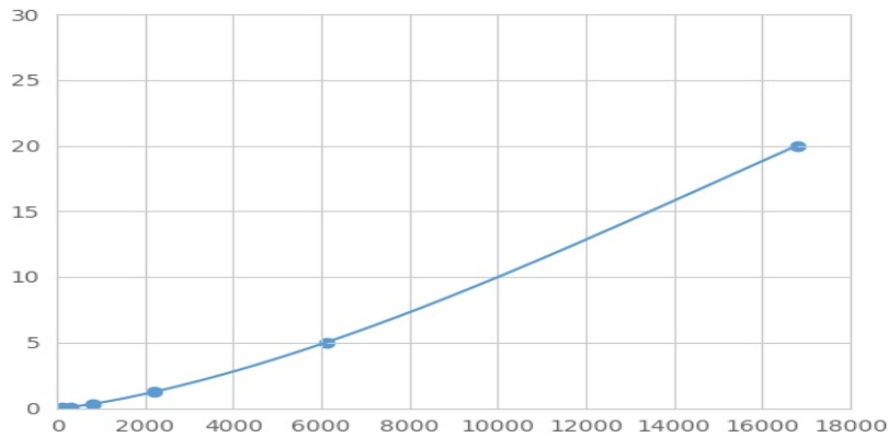
Typical Standard Curve for SIRT6 Magnetic Luminex Assay.
