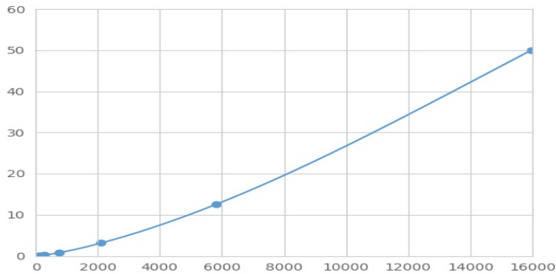
Typical Standard Curve for S100A4 Magnetic Luminex Assay.
