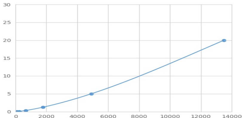
Typical Standard Curve for uPAR Magnetic Luminex Assay.
