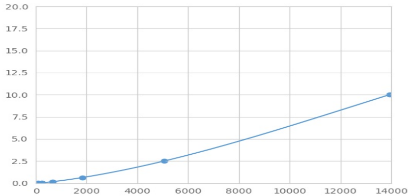
Typical Standard Curve for ITGa5 Magnetic Luminex Assay.
