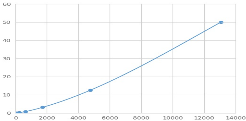
Typical Standard Curve for HDL Magnetic Luminex Assay.
