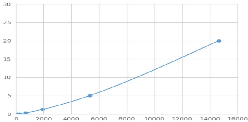
Typical Standard Curve for FOXA2 Magnetic Luminex Assay.
