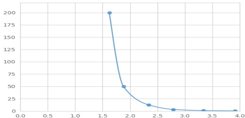
Typical Standard Curve for FS Magnetic Luminex Assay.
