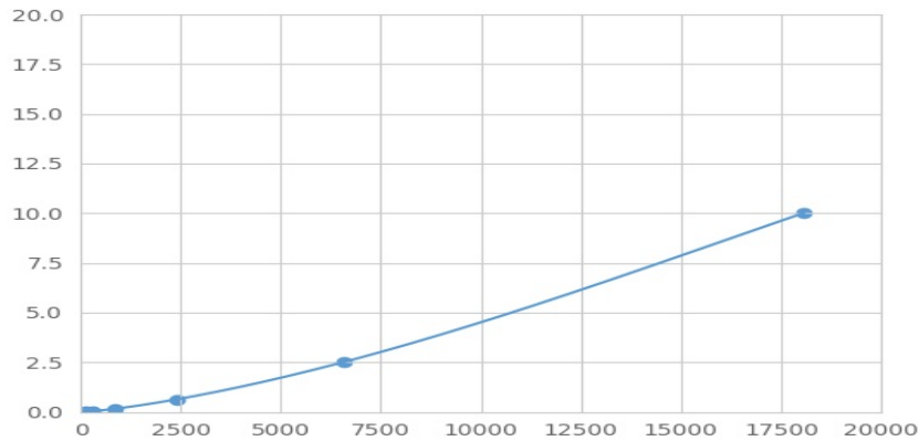
Typical Standard Curve for EAAT1 Magnetic Luminex Assay.
