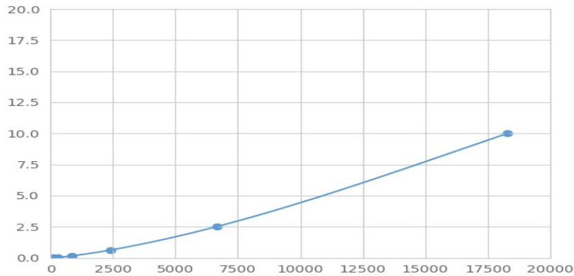
Typical Standard Curve for DCTPP1 Magnetic Luminex Assay.
