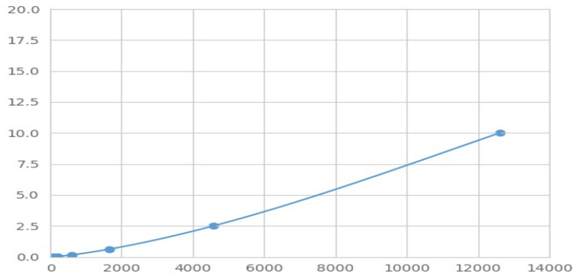
Typical Standard Curve for COL13 Magnetic Luminex Assay.
