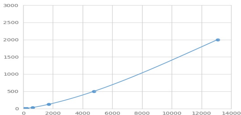
Typical Standard Curve for F7 Magnetic Luminex Assay.
