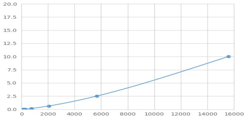
Typical Standard Curve for ADORA2b Magnetic Luminex Assay.
