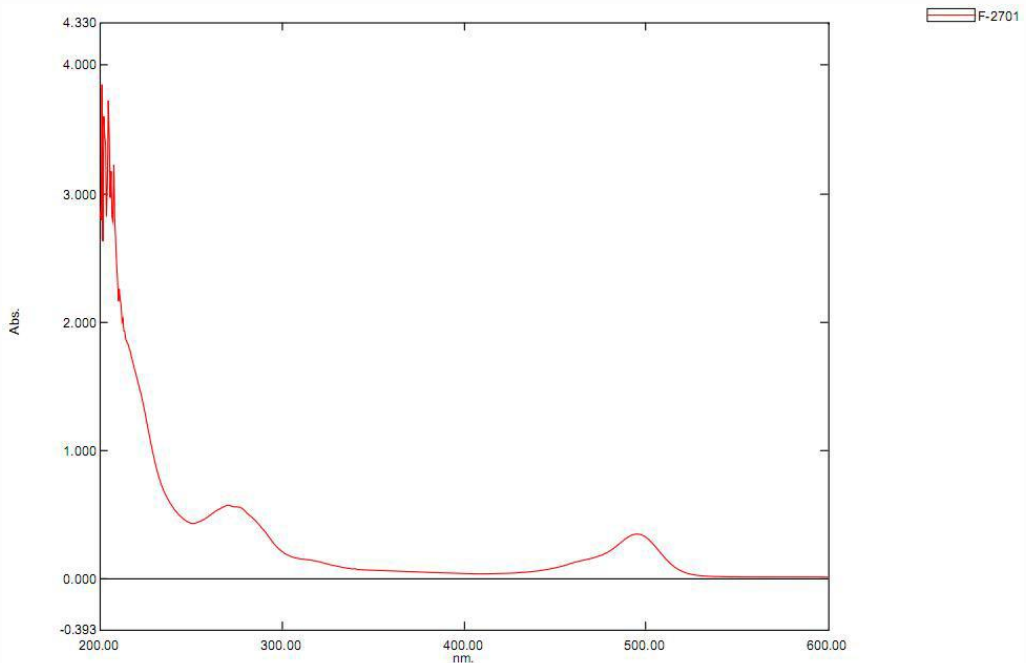
Figure 1: UV-spectrum
