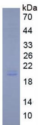
Figure 1. SDS-PAGE
