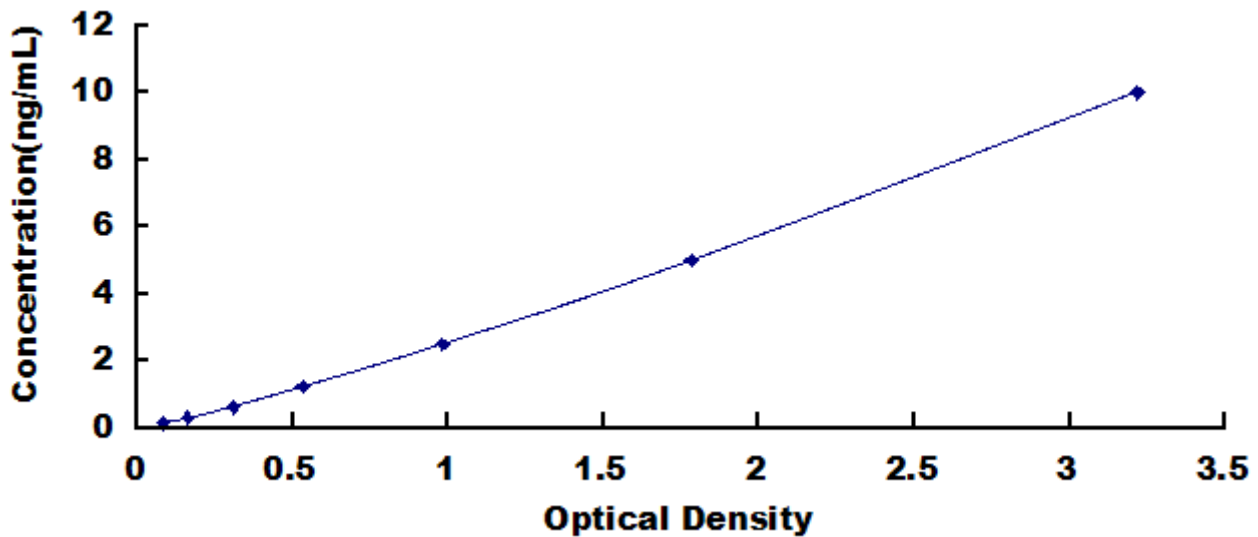
Typical Standard Curve for XYLT1, Human ELISA.
