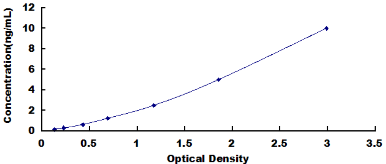
Typical Standard Curve for TLR9, Human ELISA.
