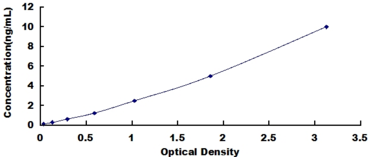
Typical Standard Curve for SORT1, Rat ELISA.
