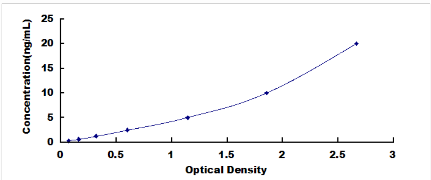
Typical Standard Curve for SOST, Human ELISA.
