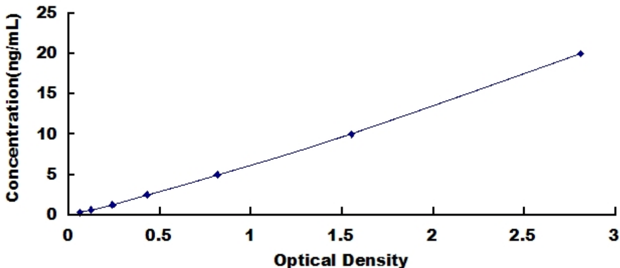
Typical Standard Curve for Resistin, Porcine ELISA.
