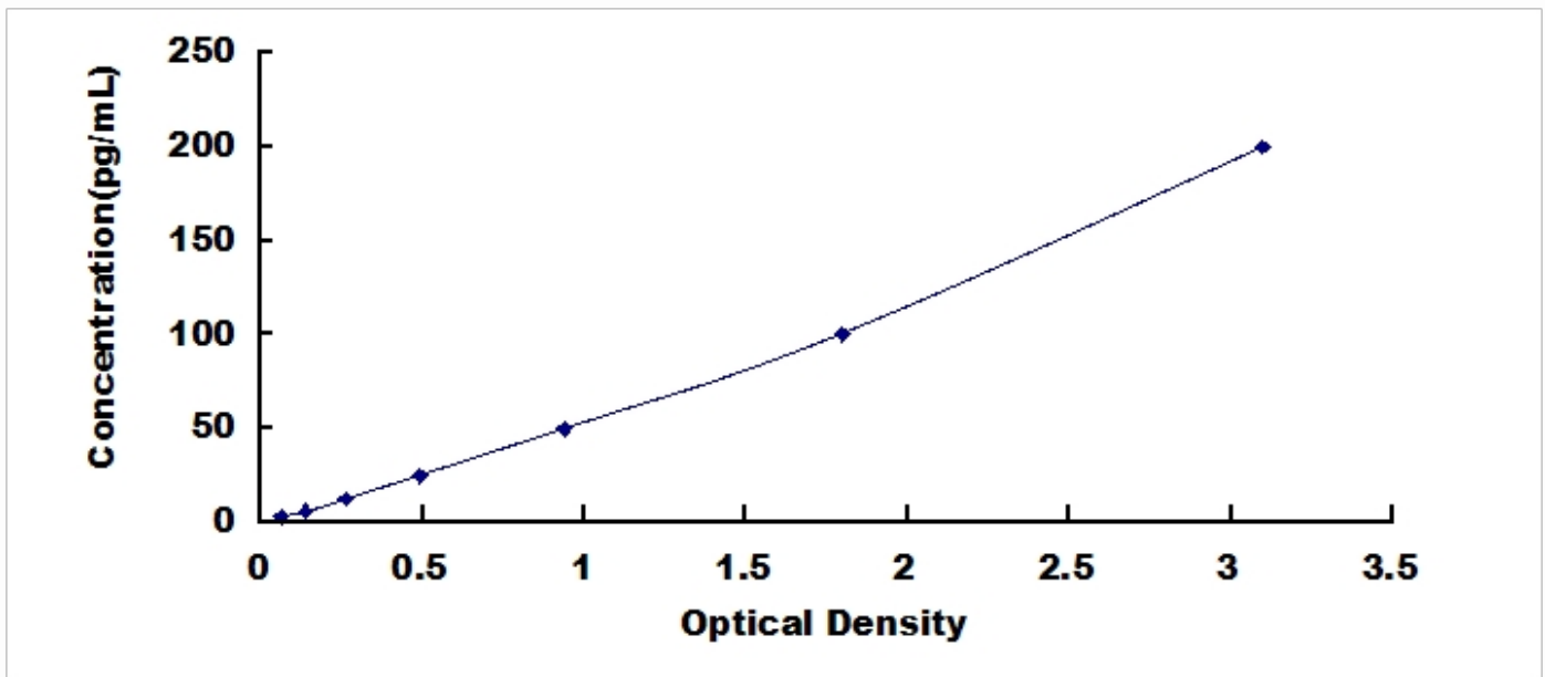
Typical Standard Curve for RANKL, Human ELISA.
