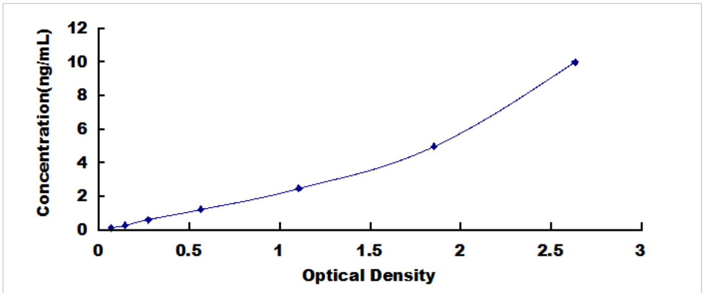
Typical Standard Curve for PPP1R15A, Mouse ELISA.
