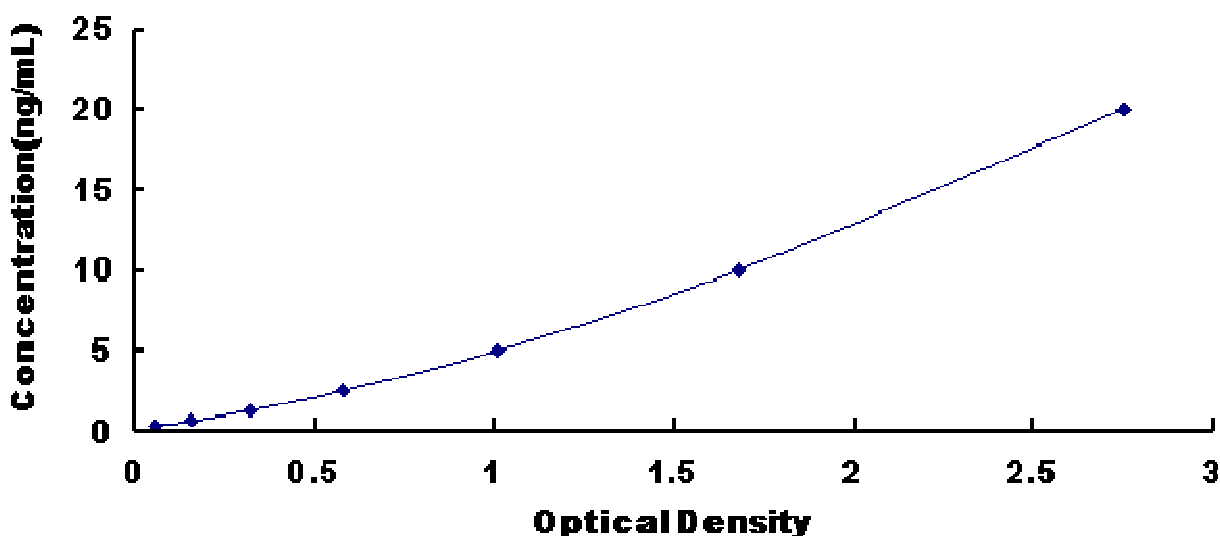
Typical Standard Curve for MMRN1, Rat ELISA.
